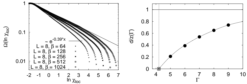
Fig. 3 Left : The integrated probability distribution of the local susceptibility \chi_i(\ln \omega = 0) of the 2d random TIFM in the Griffiths-McCoy region at \Gamma = 6.0 . The systems sizes L are larger than the spatial correlation lengths, which is small that far away from the critical point ( \Gamma > \Gamma_c \approx 4.2 ). There is, however, a dependency on the system size in the imaginary time direction, which is \beta , the inverse temperature, since here the system has long ranged correlations. Therefore \beta has to be chosen large enough to read off the correct slope of the tail of the probability distribution. Right : The value of d/z(\Gamma) obtained from analyzing the integrated probability distribution of \chi_{loc}(\ln \omega = 0) . The vertical line indicates the (approximate) region of the critical point at \Gamma_c \sim 4.2 , the open circle corresponds to z(\Gamma_c) = \infty and the horizontal line at d/z = 1 indicates the expected limit \lim_{\Gamma \rightarrow \infty} z(\Gamma) = d .
