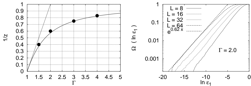
Fig. 1 Left: Exact result for the dynamical exponent 1/z(\delta) in 1d for the uniform distribution, see text ( \delta = 1/2 \ln \Gamma ). Note the asymptotic behavior at for approaching the critical point \delta \rightarrow 0 , namely 1/z(\delta) = 2\delta + \mathcal{O}(\delta^2) and the asymptotic value \lim_{\delta \rightarrow \infty} z(\delta) = 1 . The thick points are the numerical estimates obtained via the analysis of the probability distribution of the gap as it is exemplified in the right figure. Right: The integrated gap probability distribution \Omega_L(\ln \epsilon_1) in the disordered phase ( \Gamma > 1 ) for \Gamma = 2 . The dynamical exponent z(\delta) is extracted from the expected asymptotic form \ln \Omega_L(\ln \epsilon_1) = 1/z(\delta) \ln \epsilon_1 + \text{const} which is a straight line when using a logarithmic scale on the y-axis. Thus 1/z(\Gamma = 2) \approx 0.62 . Note that for large \Gamma , i.e. far away from the critical point, there is essentially no system size dependence, since the spatial correlation length is expected to be small.
