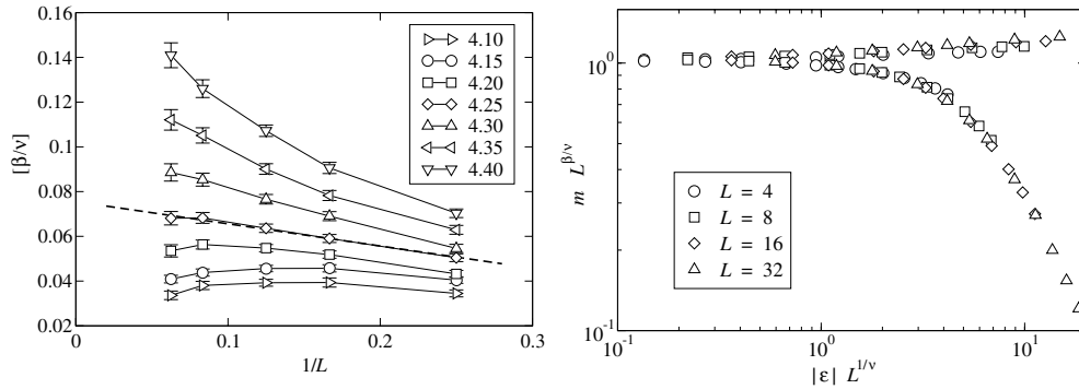
Figure 8. Left: the effective exponent [\beta/v](L) for different values of \Delta as a function of 1/L . The broken line is a guide for the eyes that separates the curves with a downward bending ( \Delta < \Delta_c ) from those with an upward bending ( \Delta > \Delta_c ). Right: scaling plot of mL^{\beta/v} versus |\epsilon|L^{1/v} with \epsilon = \Delta - 4.25 , \beta/v = 0.07 and \nu = 1.4 .
