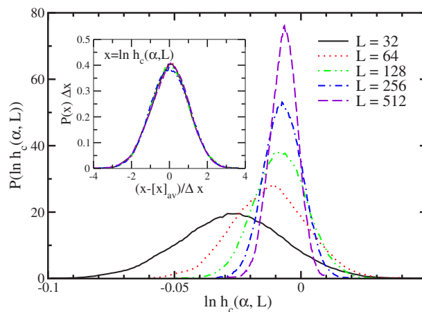
FIG. 1. (Color online) Distribution of \ln h_c(\alpha, L) for a disorder with \Delta J=0.4 , for different sizes. In the inset, the distributions of scaled variables is well described by a Gaussian.
