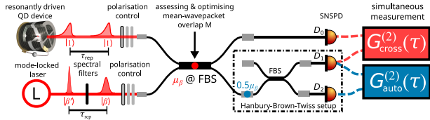
Fig.1 Setup sketch for assessing and optimizing M between single photon and coherent state..
