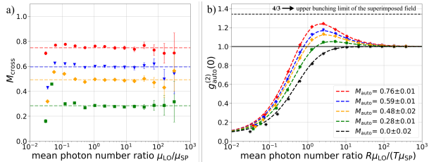
Fig.2 Measurement results from cross- and auto-correlation method. a) M_{\text{cross}} deduced from G_{\text{cross}}^{(2)}(\tau) showing the independence from \mu_{LO} . b) g_{\text{auto}}^{(2)}(\tau=0) deduced from normalizing G_{\text{auto}}^{(2)}(\tau) .
