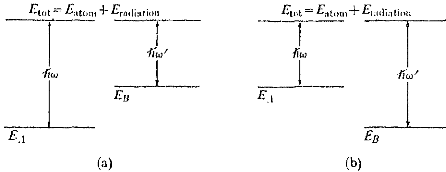
Fig. 2-4. (a) Stokes' line, (b) anti-Stokes' line.
