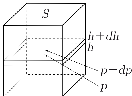
Figure 2: To derive the barometric altitude formula.
