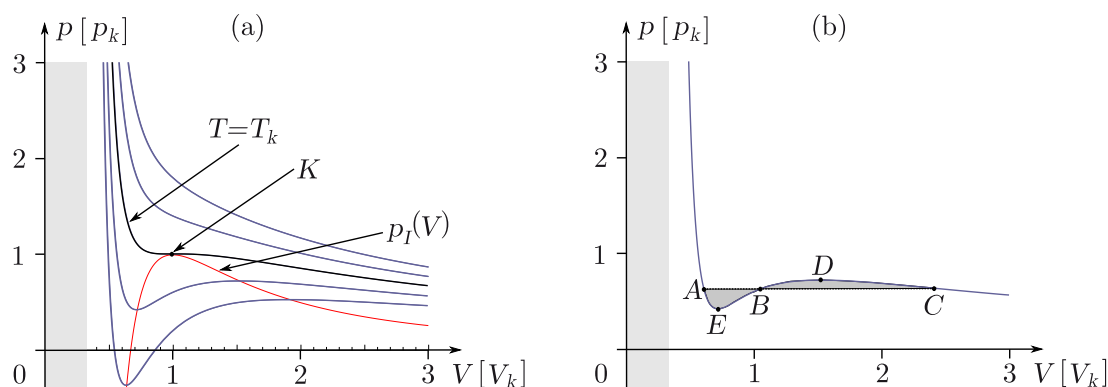
Figure 1: (a) Isotherms of the Van der Waals gas and (b) Maxwell construction.
